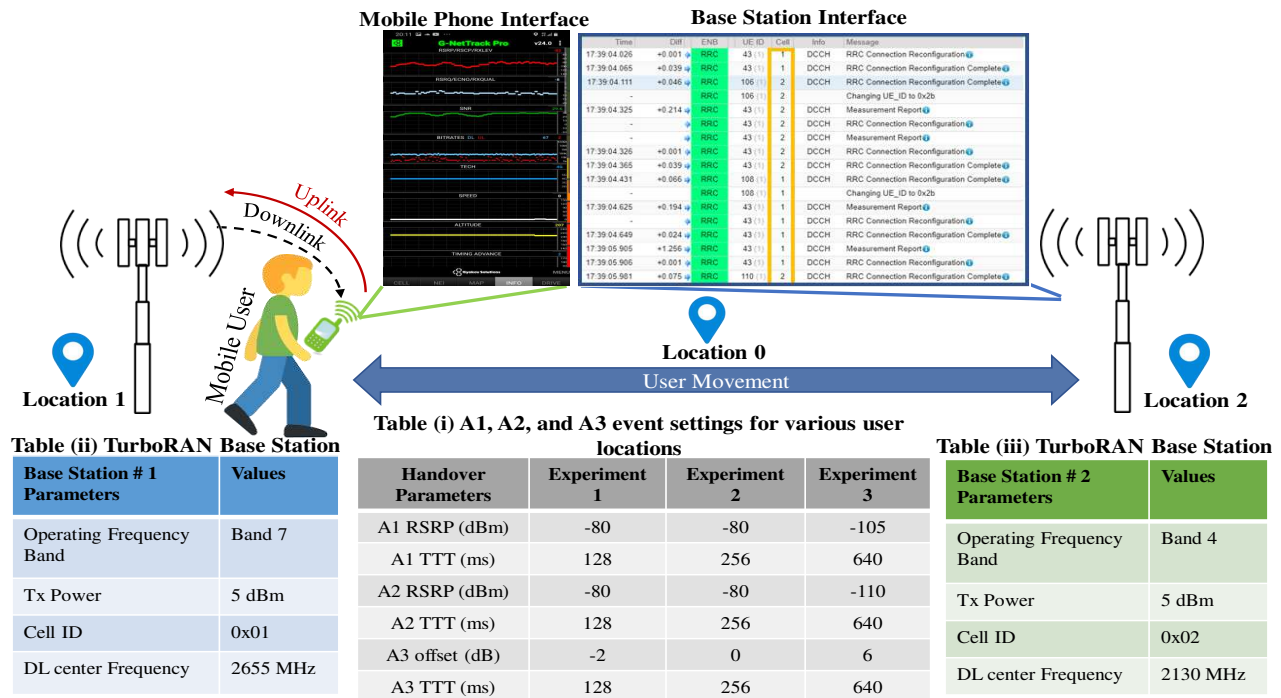
Fig. 6: Inter-frequency handover use case experimental setup.
