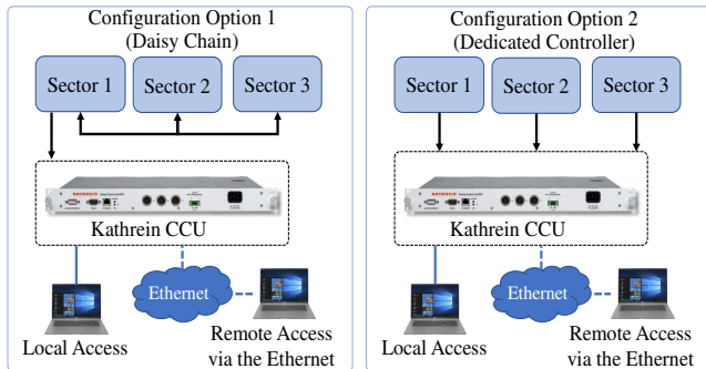
Fig. 5: Two options for RET configurations.
