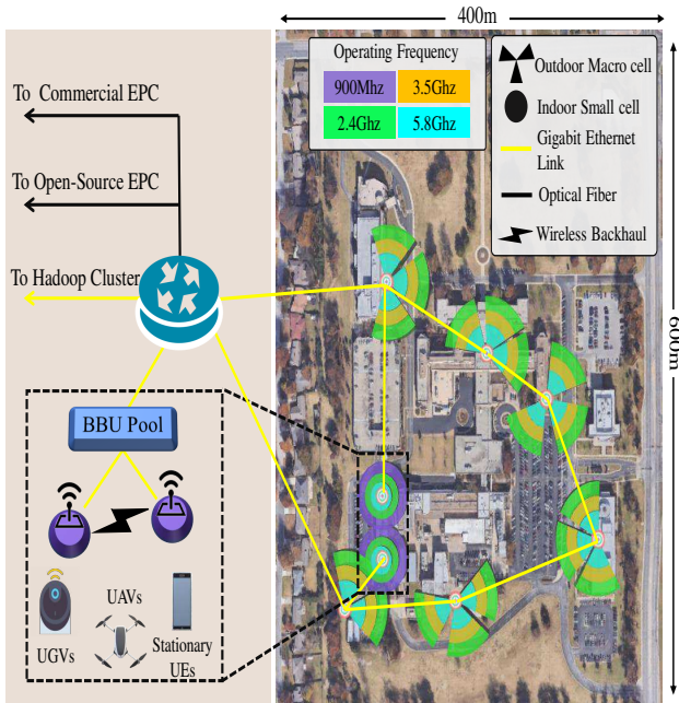
Fig. 2: TurboRAN deployment illustration.
