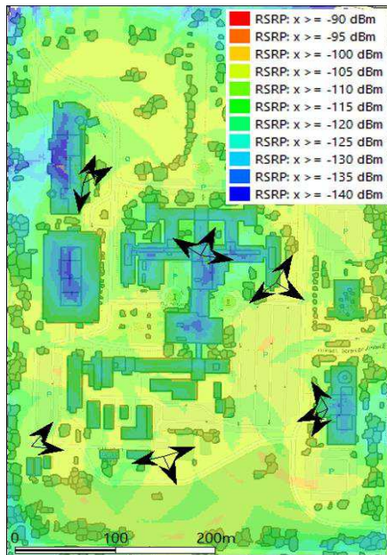
Fig. 4: Optimized RSRP simulations using Atoll.
