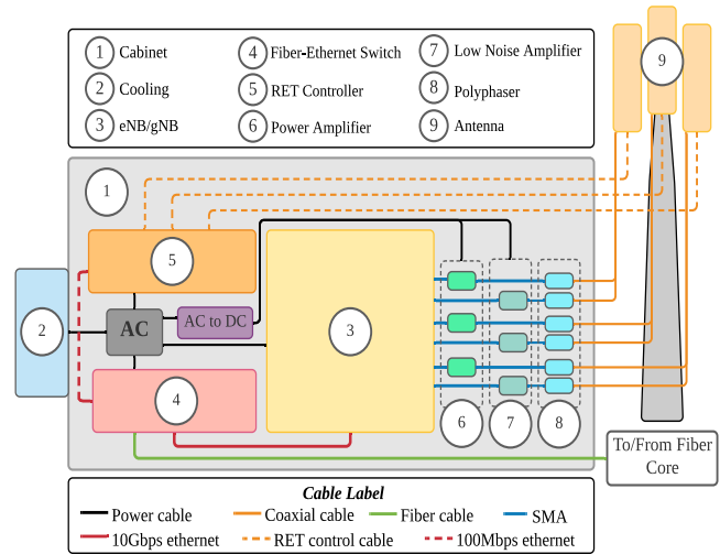
Fig. 3: Block diagram representation of the TurboRAN testbed deployment.
