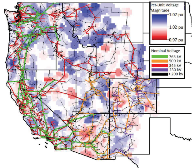
Fig. 4. Oneline diagram for the synthetic 10k case, showing the transmission lines and a voltage magnitude contour [44]. The contour shows geographically the distribution of Fig. 3, with load bus voltages varying in the range [0.97-1.07].
