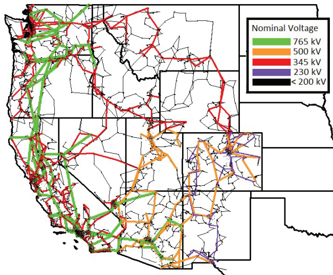
Fig. 1. Online diagram for the synthetic 10k grid, showing the transmission line voltages. This case is totally fictitious, built from public information with a synthetic methodology, and does not represent the actual grid in this location.
