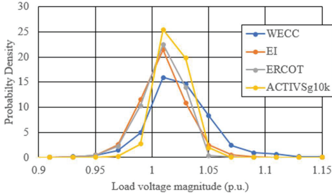
Fig. 3. Load bus voltage magnitude distribution of the synthetic 10k case (yellow) compared to the distribution found in actual cases. The EI, WECC, and ERCOT cases studied are all summer peak base planning cases, from 2012, 2013, and 2016, respectively. Although the voltage profiles can change throughout the year, the 10k synthetic case is designed to be a summer peak planning case, so it is compared to these.
