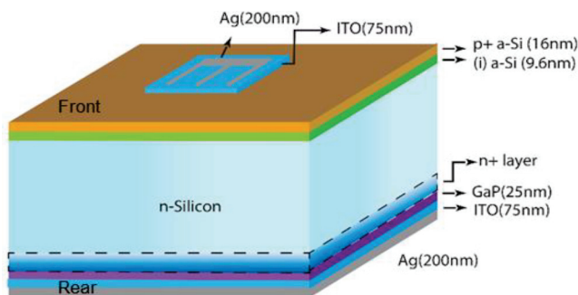
Figure 1: Schematic of a silicon heterojunction solar cell with conventional (i) a-Si/p+ a-Si front selective contact and MBE-grown GaP rear selective contact.
