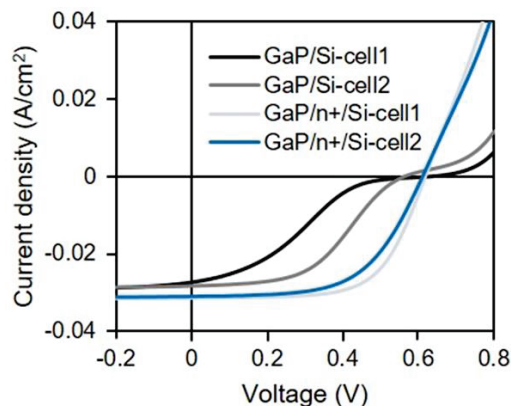
Figure 4: Current-voltage characteristics of silicon heterojunction solar cells with material stack according to Fig.1 with and without n+ doped Si layer at the GaP/Si interface for two different cells (cell1 and cell2) respectively.
