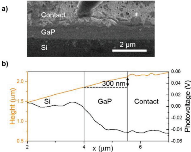
Figure 7: a) SEM image of the cross-section. b) Height and photovoltage profile across the cross-section.
