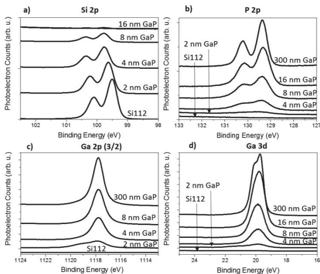
Figure 5: XPS core level spectra of GaP grown by MOCVD on Si (112).
