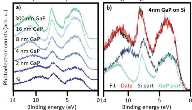
Figure 6: a) Valence band spectrum measured by XPS of Si and Si/GaP with varying GaP thickness grown by MOCVD. b) Example fit of a combined GaP/Si valence spectrum as the superposition of Si and GaP valence spectra.
