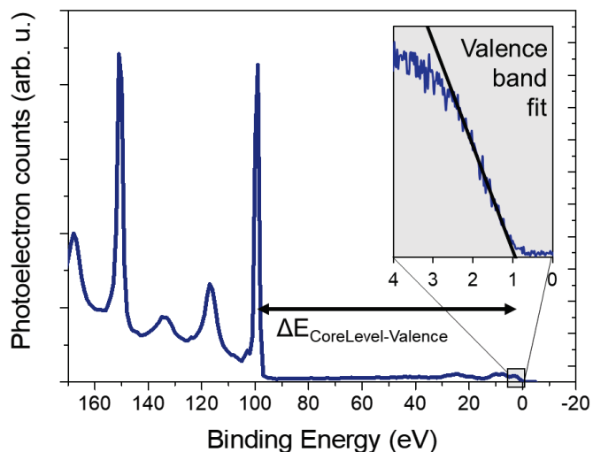
Figure 2: XPS spectrum of silicon. The inset shows a magnification of the data in the binding energy interval 0 eV-4 eV and a linear fit to the data for determination of the valence band onset.
