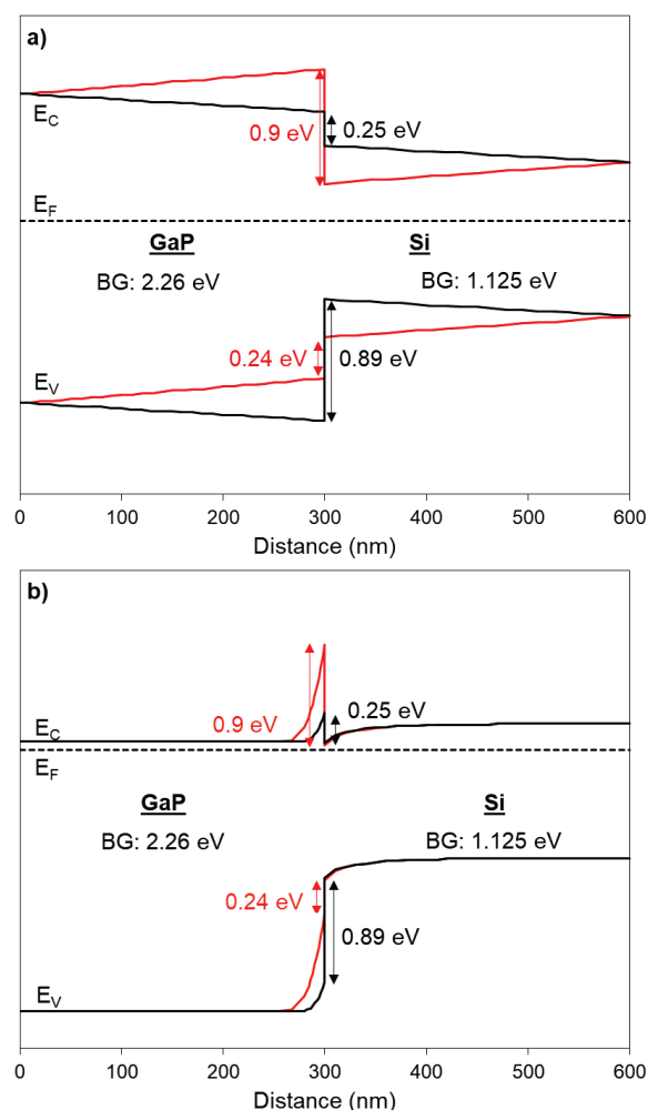
Figure 8: Band diagram for the doping level used for XPS analysis (a) and for the solar cell devices (b) as measured (red) and as predicted by Anderson's rule (black). Band diagrams were calculated using AFORS-HET v2.4.1.
