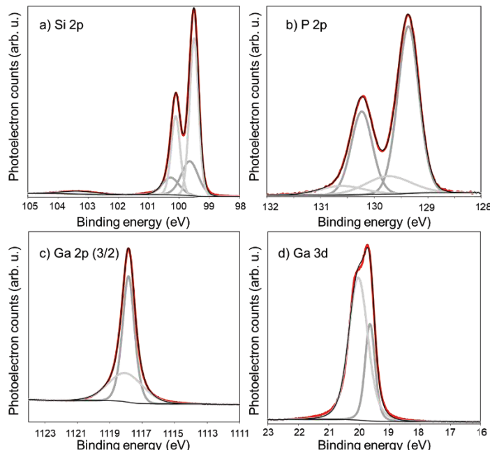
Figure 3: Core level spectra and fitting functions for a) Si 2p, b) P 2p, c) Ga 2p (3/2) and d) Ga 3d.
