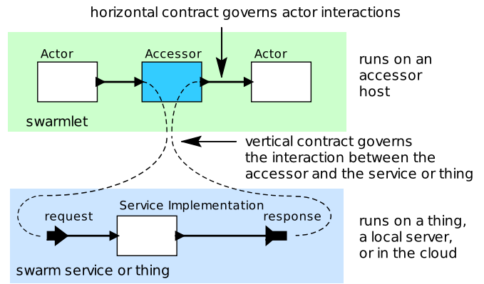
Fig. 3. Accessor in a network of actors.
