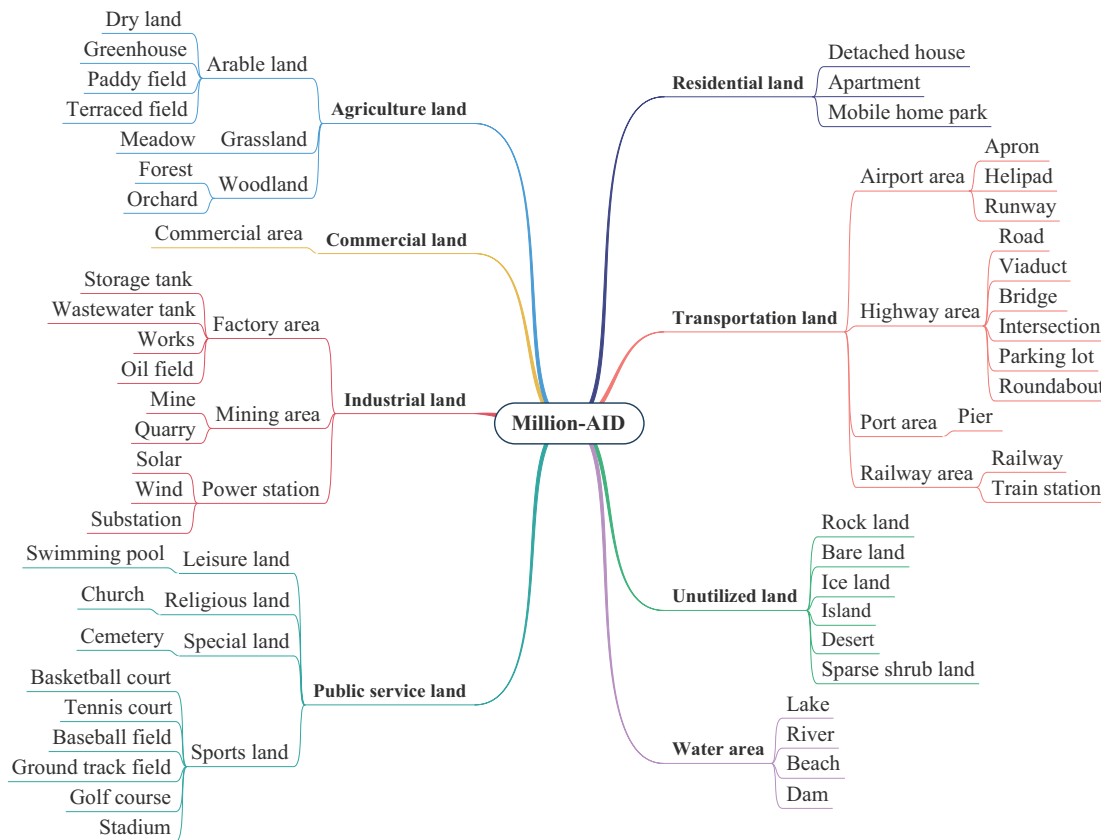
Fig. 4: The hierarchical scene category network of Million-AID. All categories are hierarchically organized in a three-level tree: 51 leaf nodes fall into 28 parent nodes at the second level which are grouped into 8 nodes at the first level, representing the 8 underlying scene categories of agriculture land, commercial land, industrial land, public service land, residential land, transportation land, unutilized land, and water area.
