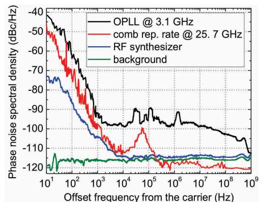
Fig. 8. Single-sideband residual phase noise of the heterodyne OPLL. Phase noise of the RF signal at 25.7 GHz generated by the comb repetition rate, RF synthesizer, and background, is also shown here for comparison.
