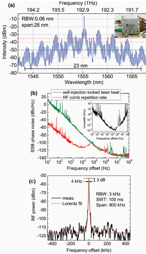
Fig. 5. (a) Optical spectrum of a stabilized Kerr frequency combs generated in the unit, as shown as inset. The comb spans 23 nm defined as defined as the spectral region in which the frequency comb envelope power exceeds -50 dBm (black dotted line) and has a line spacing of 0.2 nm, yielding more than 115 lines, being suitable for the laser phase locking. The optical output comb power exiting the fiber is 100 \mu W obtained after subtracting from the pump laser power, meaning only \sim 0.5 \mu W per comb line is achieved in the wavelength range of 1542 nm-1568 nm. The horizontal (red) dashed line denotes the \sim 0.5 \mu W per comb line power level, (b) single sideband (SSB) phase noise of the injection-locked DFB laser, used as a pump laser, integrated in the packaged OFC unit and the RF signal generated by the Kerr comb repetition rate. Extracting the instantaneous linewidth of the pump laser from its phase noise, as shown in the inset, and (c) RF beatnote, resulting from beating one of the comb lines with ultra-narrow linewidth lasers [19] to measure the optical linewidth of the comb line.
