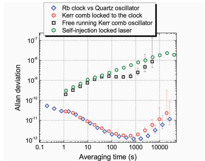
Fig. 12. The absolute stability of the locked Kerr frequency comb after locking the comb repetition rate to the Rb clock. For clarity, the result is compared it to an independent quartz ultrastable oscillator.
