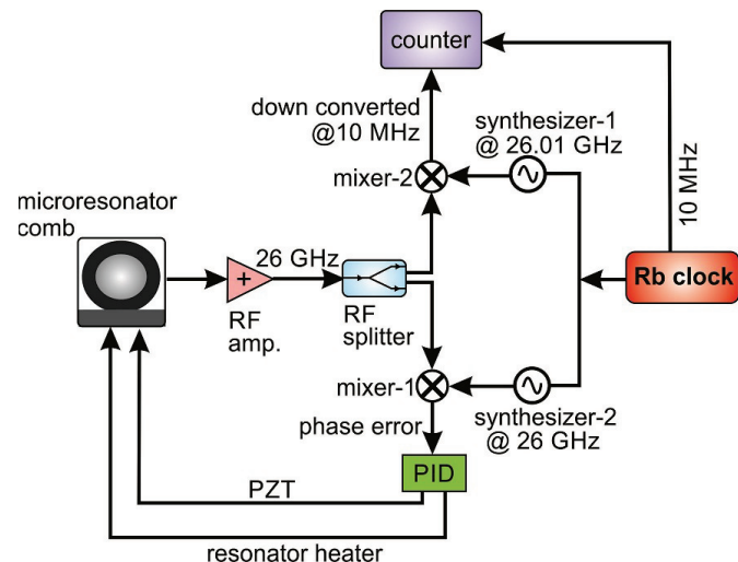
Fig. 10. The experimental setup used for locking Kerr frequency comb to a RF synthesizer. The two RF synthesizers used for phase locking of the OFC are phase locked to a rubidium clock.
