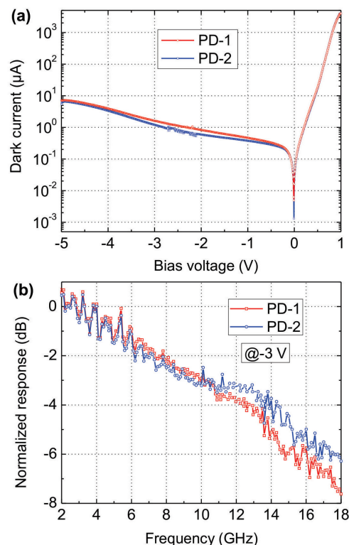
Fig 3: (a) dark currents, and (b) modulation characteristics of the two detectors in InP monolithic coherent receiver PIC. The 3-dB bandwidth is > 11 GHz.
