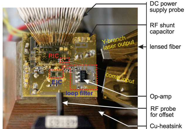
Fig. 4. Microscope image of the entire heterodyne OPLL system where PIC, COTS ICs and loop filter are highly integrated on a separate AlN supercarrier. Finally, it rests on a copper heatsink for the measurement. Two lensed fibers at the right are butt-coupled to the waveguide endface of the photonic chip.
