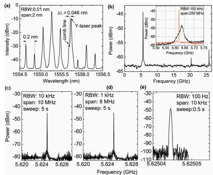
Fig. 7. (a) Optical spectrum when Y-branch laser is offset-locked to the comb at 1555.69 nm with a wavelength difference of 0.046 nm, (b) RF spectrum of the locked beatnote between Y-branch laser and comb at 5.6 GHz is recorded. The beatnote generated between on-chip laser and adjacent comb line at 20.1 GHz and the beatnote produced between comb lines at 25.7 GHz are also visible. The resolution bandwidth is 3 MHz. The zoom-in spectra with a span of 250 MHz is shown as inset where the phase-locked (red) and free-running (black) cases can be seen, and (c)-(e) measured RF beatnotes at various RBWs.
