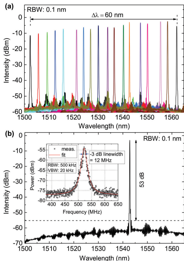
Fig. 2. (a) Superimposed measured lasing spectra of the Y-branch laser with an emission wavelength, ranging from 1502 to 1562 nm, and (b) typical single-mode lasing spectrum at a wavelength of ~1543 nm with a side-mode suppression ratio of 53 dB. Beat spectrum of the laser obtained using a heterodyne technique is shown as inset.
